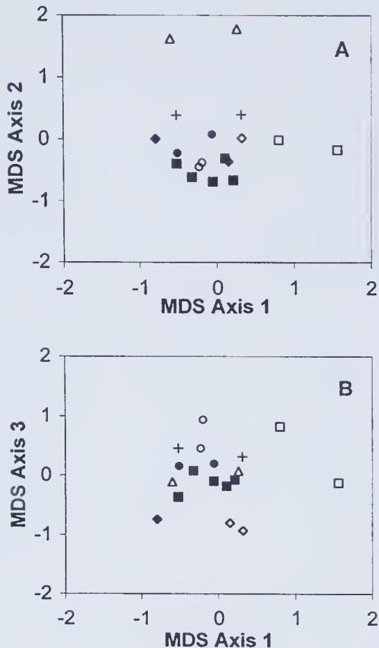
Figure 5. Three-dimensional ordination of waterbird surveys from Toolibin Lake (presalinity, \blacklozenge ; baseline, \blacksquare ; 1996, \bullet ), Walbyring Lake (o), Lake Chandala ( \diamond ), Lake Cooloongup ( \Delta ), Lake Eganu ( \square ) and a small wetland (+) on the eastern edge of Watheroo National Park (see text for details), showing separation of Eganu, Cooloongup and Chandala from the other, Casuarina obesa -dominated wetlands; stress = 0.14.
